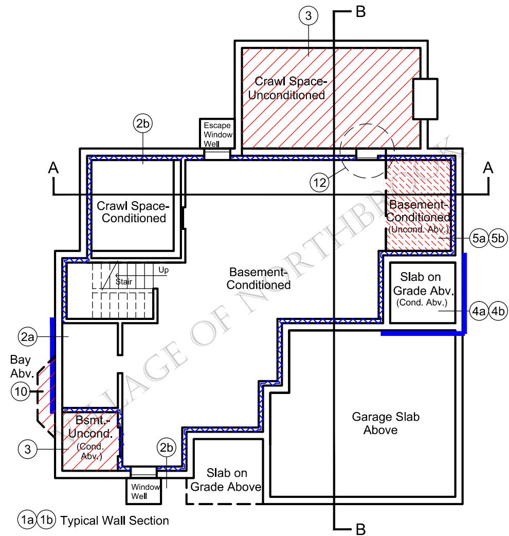
Basement / Foundation Energy Plan
