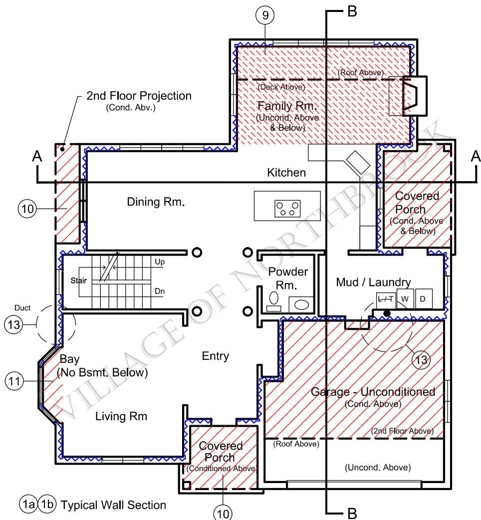
1st Floor Energy Plan
